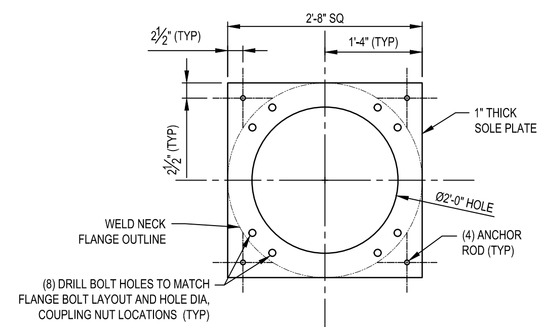
C DETAIL - SOLE PLATE SCALE: 3/4" = 1'-0"
