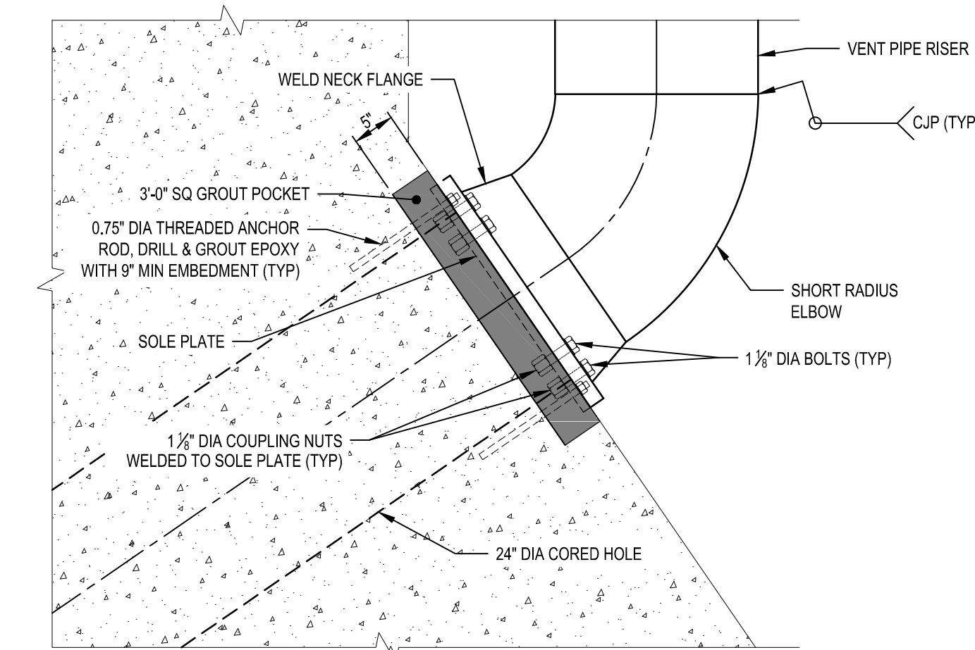
A DETAIL - SIPHON VENT BASE SCALE: 3/4" = 1'-0"
