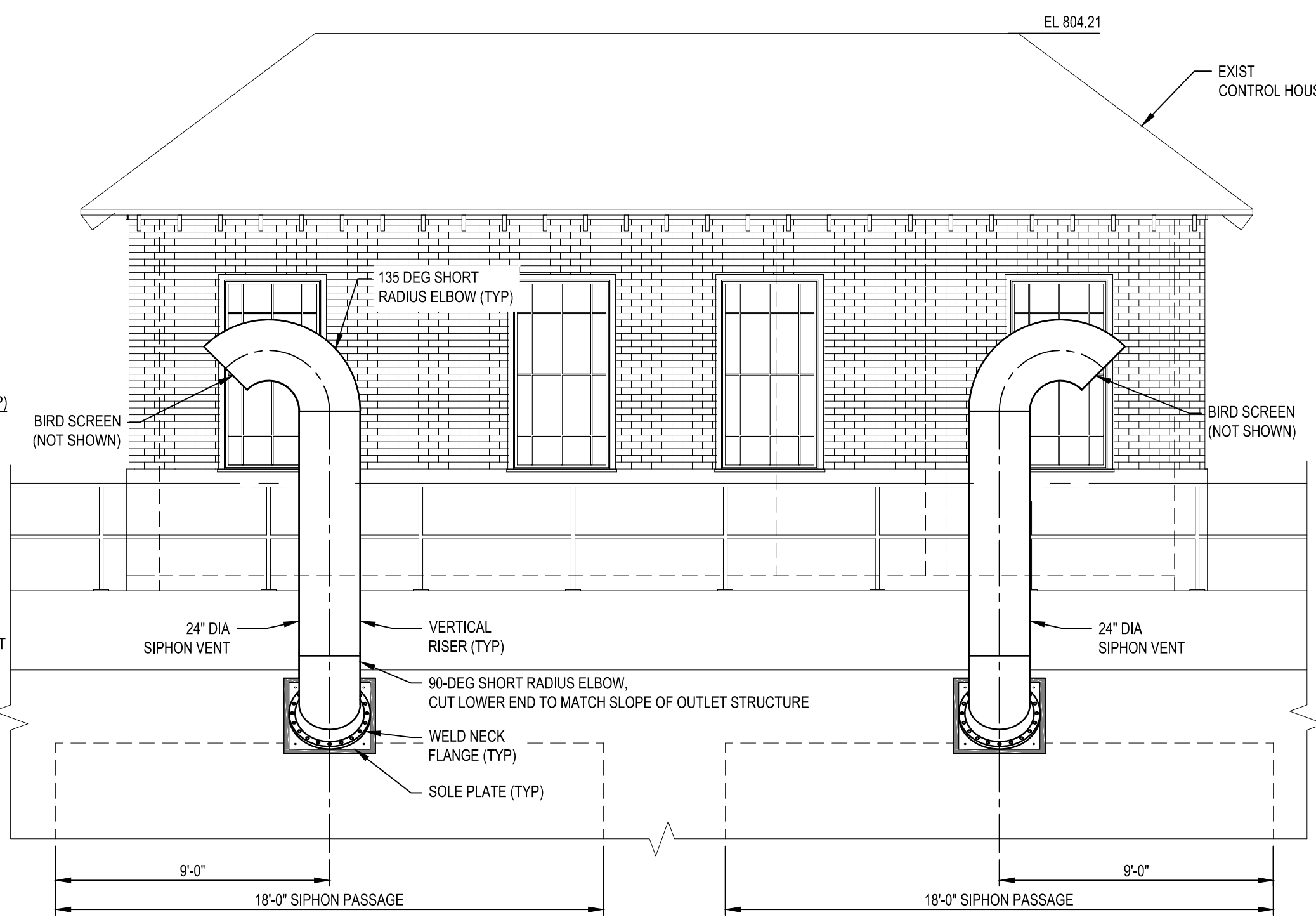
2 DOWNSTREAM ELEVATION SCALE: 1/4" = 1'-0"
